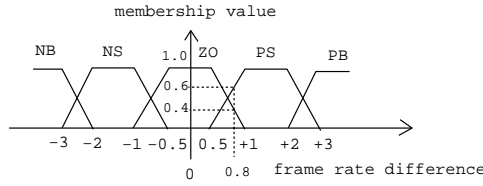
Fig. 5. Membership functions for the input: frame rate difference
