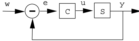
Fig. 1. A feedback control system
