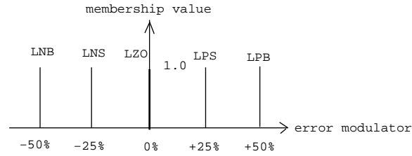
Fig. 7. Output singleton membership functions for error modulator
