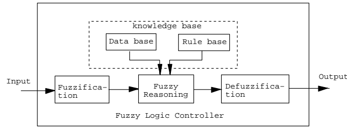
Fig. 3. Principal components of a fuzzy logic control system
