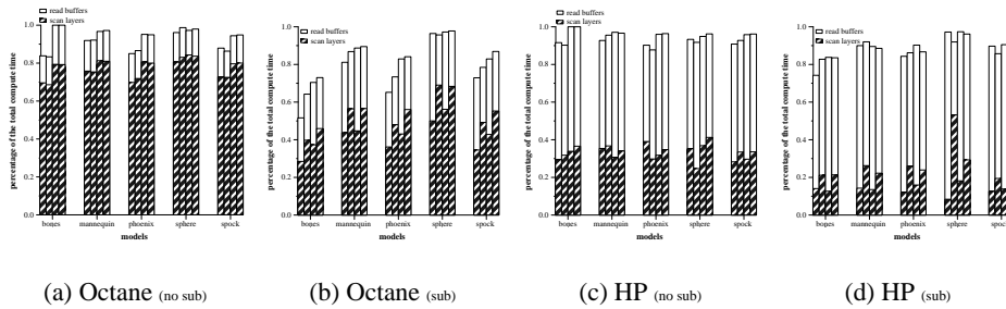
Fig. 2. Percentage of the overall execution time spent on scanning layers and reading frame buffers of the algorithm with and without the subdivision scheme on Octane and HP.
