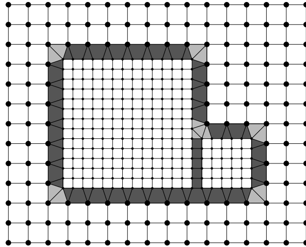
Fig. 3. “Stitch cells” for first two levels of AMR data set shown in Fig. 2
