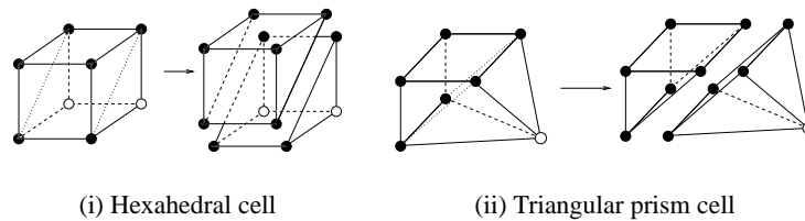
Fig. 6. Tessellations for 3D cells
