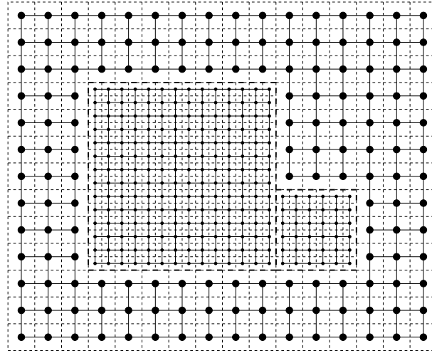
Fig. 2. Dual grids for the three AMR grids comprising the first two hierarchy levels shown in Figure 1. The original AMR grids are drawn in dashed lines and the dual grids in solid lines
