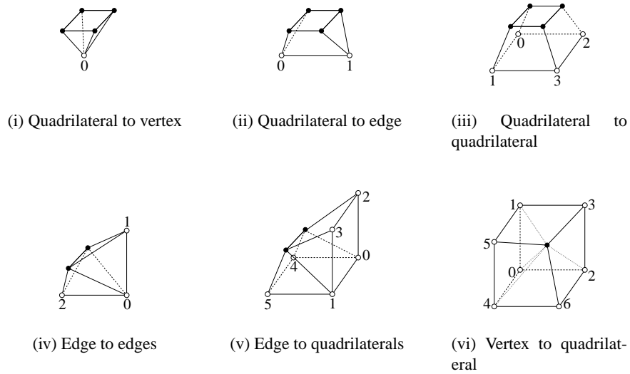
Fig. 5. Possible connection types for quadrilateral, edge and vertex in 3D case
