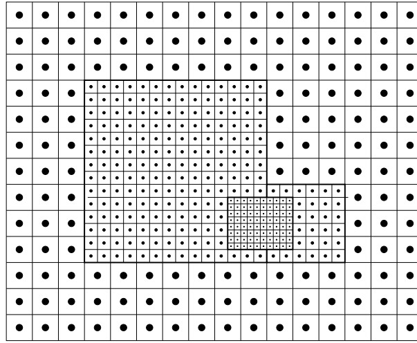
Fig. 1. AMR hierarchy consisting of four grids in three levels. The root level consists of one grid. This grid is refined by a second level consisting of two grids. A fourth grid refines the second level. It overlaps both grids of the second level. Boundaries of the grids are drawn as bold lines. Locations at which dependent variables are given are indicated by solid discs
