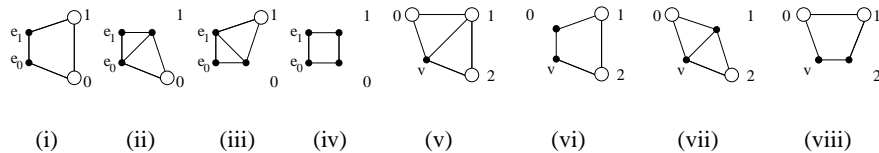
Fig. 4. Possible cases for connecting a boundary edge \overline{e_0e_1} ((i)–(iv)) or a boundary vertex v ((v)–(viii)) to a coarse grid. If cells of the coarse grid are refined, the coarse grid points (circles) are replaced by the corresponding refining point (solid black discs)
