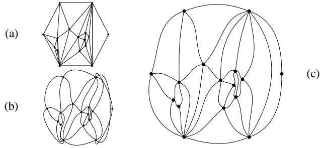
Fig. 5. A straight-line triangulation (a) and curved edges in a balanced rotation (b). Using the half-sided templates of Fig. 4 for vertices on the convex hull significantly improves the drawing (c)
