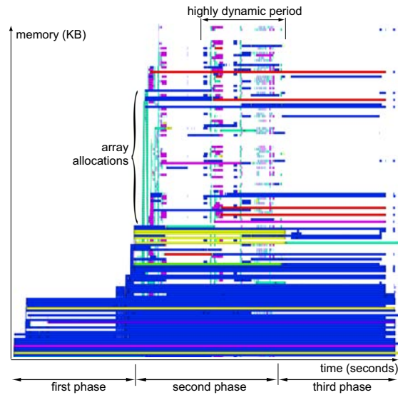
Figure 1: Dynamic memory allocation visualization
