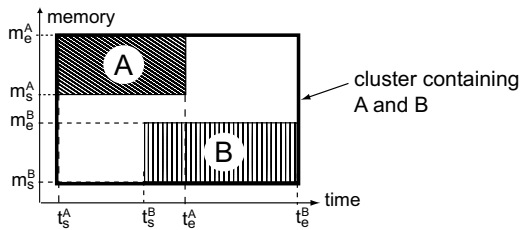
Figure 4: Distance metric construction
