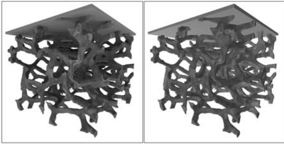
Figure 5: Compaction of foam by a rigid plate. The foam sample is about 1 \text{ mm}^3 . The initial geometry was collected using micro-CT, which was then converted to a particle distribution, thus bypassing the extreme difficulties associated with constructing a suitable body-fitted mesh [BBMS06]. The left image includes ambient occlusion shading texture values. The image on the right contains direct lighting only. It took 12 hours to precompute the textures. Frame rates to render the left and right images (500x500) were 7.35 f/s and 8.67 f/s respectively. (Color version Figure 13.)
