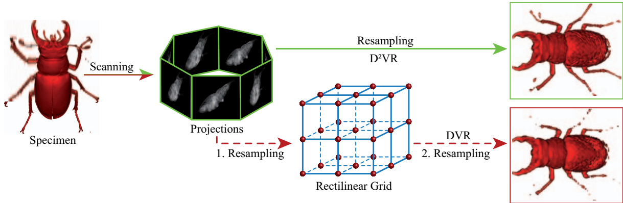
Figure 2: Data processing work flow of projection- and grid-based volume rendering. The dashed line corresponds to the traditional volume rendering pipeline. It requires two resampling steps in order to visualize the data. First an intermediate grid is resampled and then this grid is resampled again during ray traversal. The solid line corresponds to the projection-based volume rendering pipeline; one lossy resampling step is avoided.
