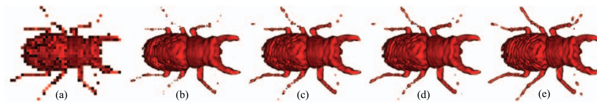
Figure 1: CT scan with insufficient resolution of a stag beetle as specimen. Figure (a) to (d) show DVR using different reconstruction schemes: (a) using nearest neighbor reconstruction, (b) using trilinear-, (c) using Catmull-Rom-, and (d) using polynomial interpolation of degree five. (e) shows D 2 VR of projection-based volumetric data. Figure (a) - (d) were rendered from grids with a resolution of 64^3 . Figure (e) was rendered from 64 projections each with a resolution of 64^2 .
