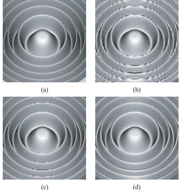
Figure 5: Comparison of an iso-surface of the Marschner & Lobb function: (a) Analytically computed. (b) DVR rendering of a 64^3 grid. (c) DVR rendering of an eight times bigger grid ( 128^3 ). (d) D 2 VR from projection-based volumetric data (64 projections, each projection with a resolution of 64^2 ). Grids are reconstructed from 64 filtered projections, each projection with a resolution of 64^2 .
