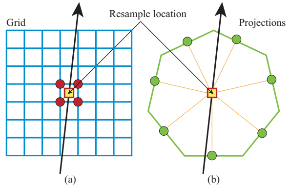
Figure 3: Difference of grid-based and projection-based resampling. (a) illustrates resampling along a ray on rectilinear volumetric data and (b) shows resampling along a ray directly from the filtered projections.
