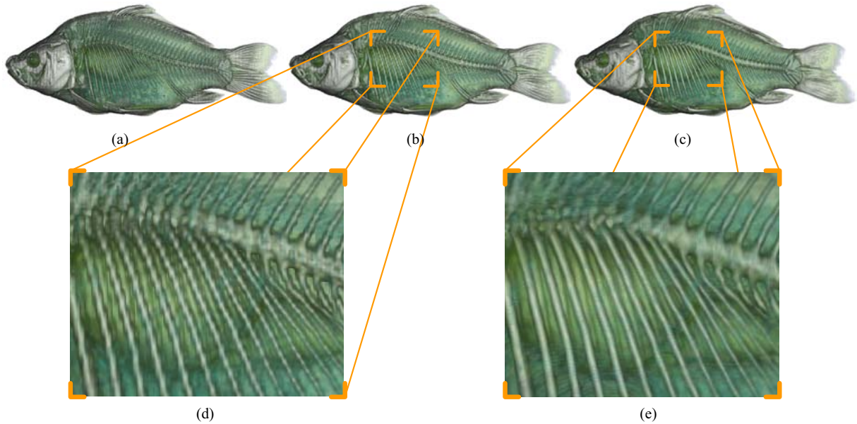
Figure 6: CT scan of Carp (256x256x512): (a) DVR of original grid. (b) DVR of a 128x128x256 grid, reconstructed from 128 filtered projections, each projection with a resolution of 128x256. (c) D^2VR of projection-based volumetric data (128 projections, each projection with a resolution of 128x256). (d) close-up of DVR. (e) close-up of D^2VR .
