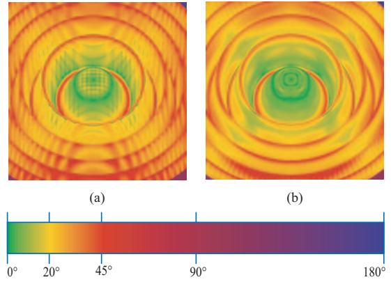
Figure 9: Color encoded differences in degrees between analytically computed gradients and (a) the estimated gradients using central difference gradient estimation on the grid, (b) the estimated gradients using our new projection-based gradient estimation method.
