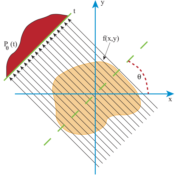
Figure 4: Parallel projection for a specific angle \theta .
