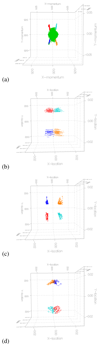
Figure 5: Tracking particle motion over time in a 500 time step beam injector simulation. (a) The p_x p_y p_z -plot of the full distribution in time step 500, at the end of the simulation, where four jets of particles are clearly visible and have been selected in four distinct groups, each with its own color. Figures (b), (c), and (d) show xyz -plots of time steps 90, 370, and 500, respectively, of the four selected groups, the core of the beam being rendered invisible. Note that each group remains in a tight formation even though heavy particle mixing is occurring, but is spread over multiple beamlets.
