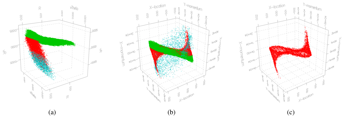
Figure 4: Correlating points across different views of the same data. An integrated beam experiment (IBX) data set represents a beam after it has undergone significant phase space distortion. (a) An Rv_Rv_\Theta -plot of a polar coordinate version of the data is plotted in Cartesian coordinates. R denotes the radial coordinate, v_R the velocity of R , and v_\Theta the velocity of the angular coordinate \Theta . A typical “hoe”-shaped distribution is observed. (b) The corresponding xp_xp_y -plot of a Cartesian coordinate version of the data is plotted. (c) Attention is brought to the interesting shape representing the effects of strong anharmonic forces in the xp_xp_y -plot by making selections other than the red selection invisible.
