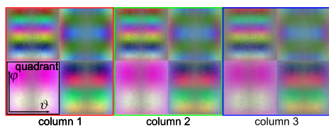
Figure 5: The BRDF coefficient texture for the aluminum-bronze material. One quadrant holds 4 coefficients for each \omega_o . The x -axis spans the values \vartheta = 0 \dots \pi and the y -axis the values \varphi = 0 \dots 2\pi .
