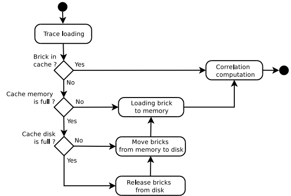
Figure 4: Classic cache system mechanism. Bricks that contain voxels with the highest correlation are kept in the cache.
