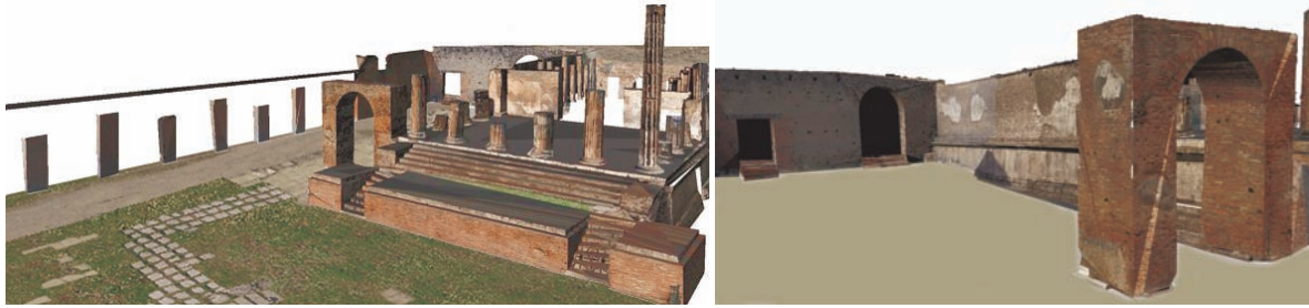
Figure 4: The first results of the integration of different image- and range-based 3D models of finds and large mural structures (Zeus temple's area).
