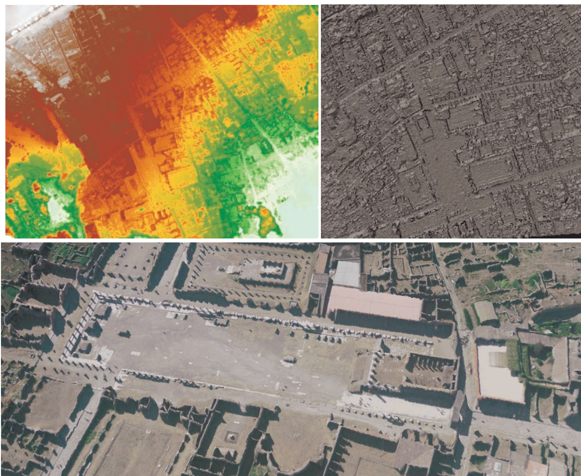
Figure 2: The DSM (18 Mil points) of the archaeological area of interest (ca 1x0.8 km) generated from three aerial images, shown in colour-code and shaded mode (above). A closer view of the textured model of the Forum (25 cm geometric resolution).
