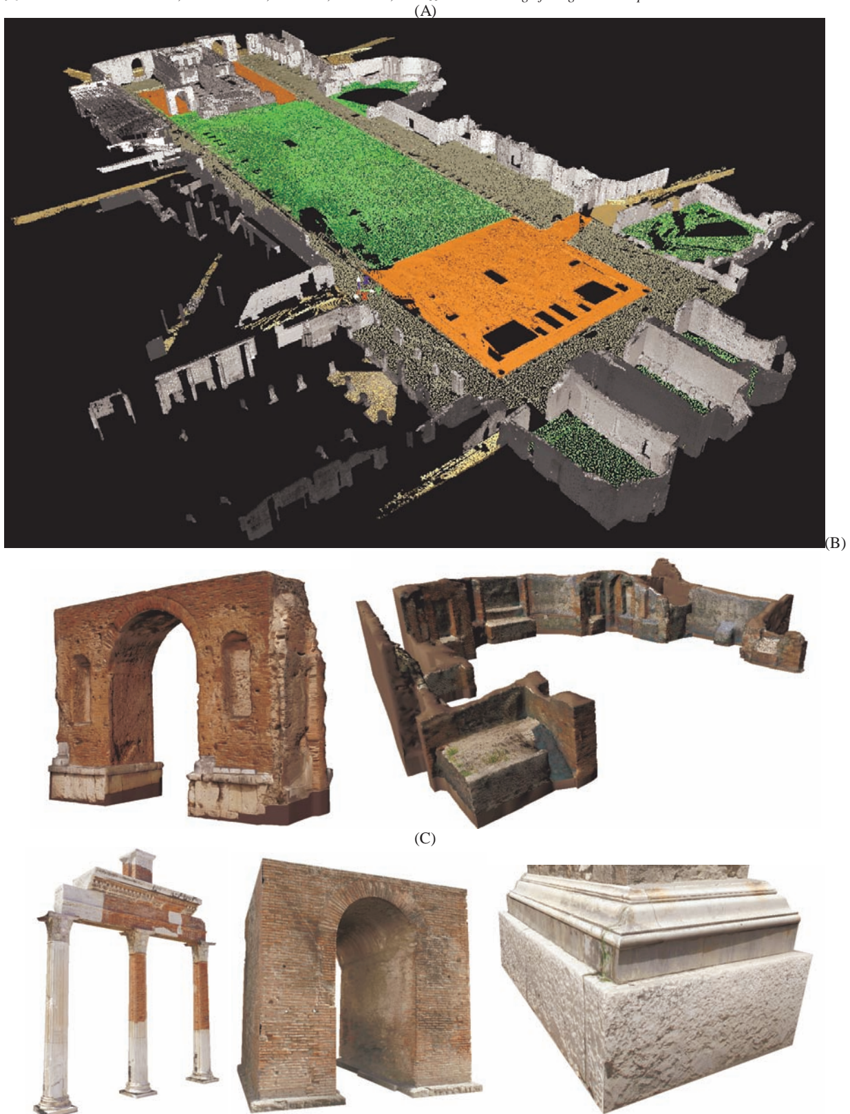
Figure 3: Range data of the main mural structures of the Forum (A), range models of archeologically interesting large structures(B) and terrestrial photogrammetric models of columns, arches or finds (C).
