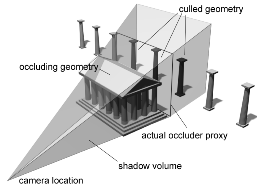
Figure 6: Shadow Culling technique for eliminating non-visible polygons in the viewing frustum.
