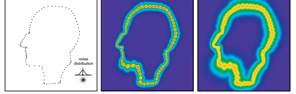
Figure 6: The effect of noise on the likelihood map. Left: Input point cloud, middle: Likelihood map without noise, right: Likelihood map with identically distributed Gaussian noise.
