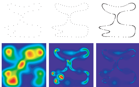
Figure 8: Adaptive surface sampling. A given continuous surface has been successively up-sampled by inserting points in regions of low confidence. The bottom row shows the confidence map of the corresponding point clouds shown in the top row.
