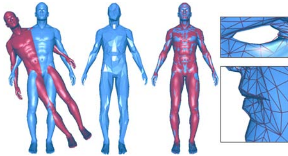
Figure 7: Quasi-Rigid Prior using Multiresolution: Matching two full body meshes with different sampling ( \sim 28K vertices each) by minimizing their Hausdorff distance with a quasi-rigid gradient flow. To speed up computations, a multi-resolution scheme was employed (total time: 1 min). The coarsest resolution is shown in the middle. Closeups show the final alignment (template mesh in wireframe).
