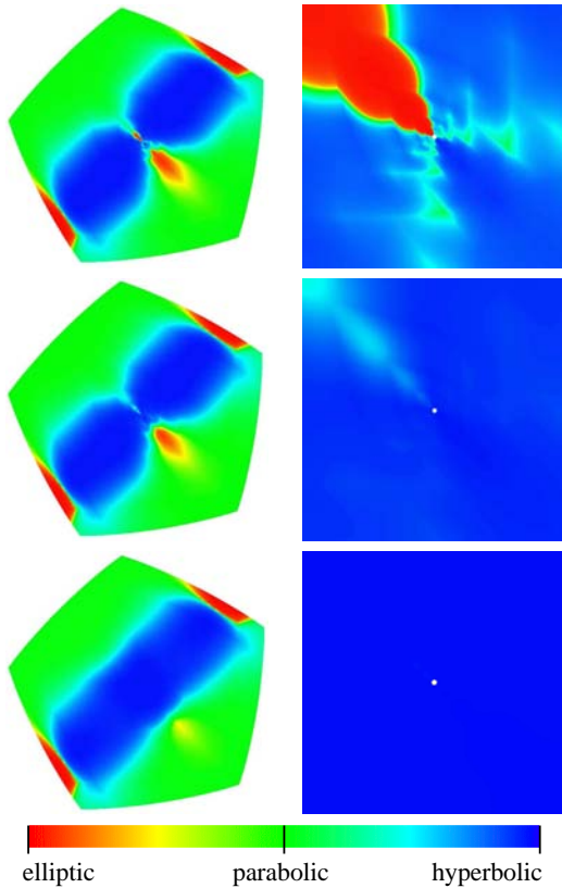
Figure 6: Visualization of the Gauss curvature of the uncorrected hybrid surface (top) of Figure 4, the surface generated with slow correction to a hyperbolic shape with \alpha = 0.95 in every step (middle) and the surface generated with fast correction to a hyperbolic shape with \alpha = 0.0 (bottom). The right column shows the corresponding zoom-in at the extraordinary points after 10 subdivision steps.
