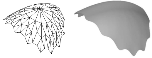
Figure 5: A control-net with a 15-valent vertex and the corresponding hybrid surfaces generated by the bounded curvature variant of Loop's algorithm.
