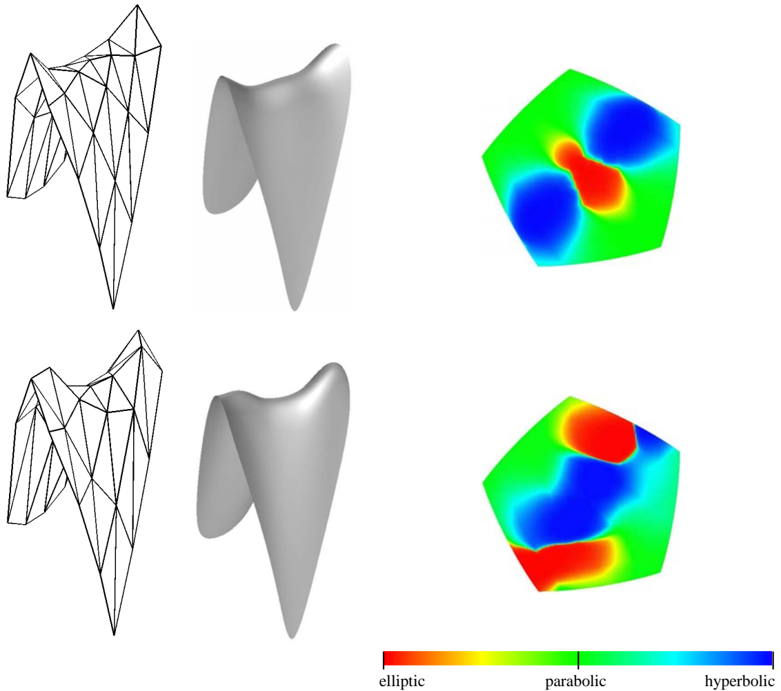
Figure 10: Control-net, flat-shaded surface and visualization of the Gauss curvature of the surface corresponding to the surface in Figure 4 corrected to an elliptic shape using \kappa_3 = 0.12, \kappa_4 = \kappa_5 = 0 (top) and to a hyperbolic shape using \kappa_3 = 0, \kappa_4 = \kappa_5 = 0.12 (bottom) with the two-ring neighborhood extension. The right column shows the zoom-in at the extraordinary points after 10 subdivision steps. Compare with the control-nets and flat-shaded surfaces in Figures 4 and 8 and the visualization of the Gauss curvature in Figures 6 (top) and 8.
