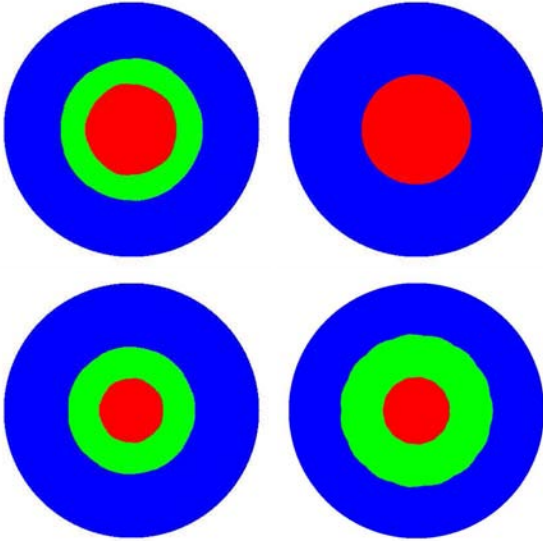
Figure 2: Shape charts in polar coordinates for the bounded curvature variant of Loop's algorithm of Section 3 for valences 5, 6, 7 and 15. Red encodes elliptic, green hybrid and blue hyperbolic shapes.
