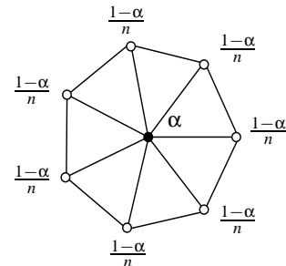
Figure 3: The stencil for the correction.
