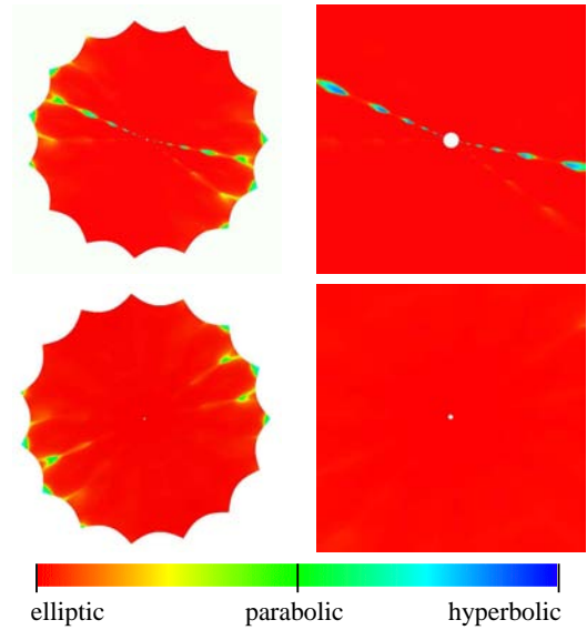
Figure 7: Visualization of the Gauss curvature of the uncorrected hybrid surface (top) of Figure 5 and the surface generated with correction to an elliptic shape with \alpha = 1.2 in the first three steps and no correction in the subsequent steps (bottom). The right column shows the corresponding zoom-in at the extraordinary points after 10 subdivision steps.
