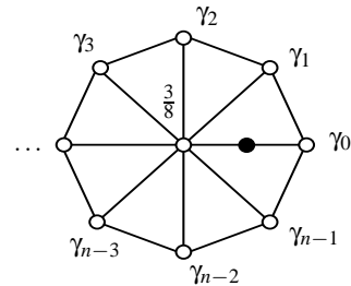
(c) The additional stencil of the bounded curvature variant of Loop's algorithm for edge-points near a vertex of valence n .
