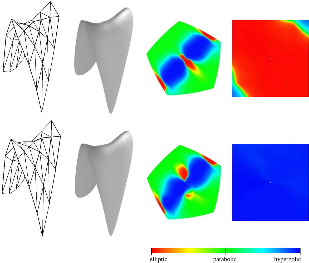
Figure 8: Control-net, flat-shaded surface and visualization of the Gauss curvature of the surface corresponding to the surface in Figure 4 corrected to an elliptic shape using \kappa_3 = 0.12, \kappa_4 = \kappa_5 = 0 (top) and to a hyperbolic shape using \kappa_3 = 0, \kappa_4 = \kappa_5 = 0.12 (bottom). The right column shows the zoom-in at the extraordinary points after 10 subdivision steps. Compare with the control-net and flat-shaded surface in Figure 4 and the visualization of the Gauss curvature in Figure 6 (top) of the surface with hybrid shape.
