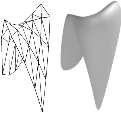
Figure 4: A control-net with a 5-valent vertex and the corresponding hybrid surfaces generated by the bounded curvature variant of Loop's algorithm.
