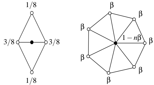
(a) The stencil of Loop's algorithm for edge-points. (b) The stencil of Loop's algorithm for vertex-points of valence n .
