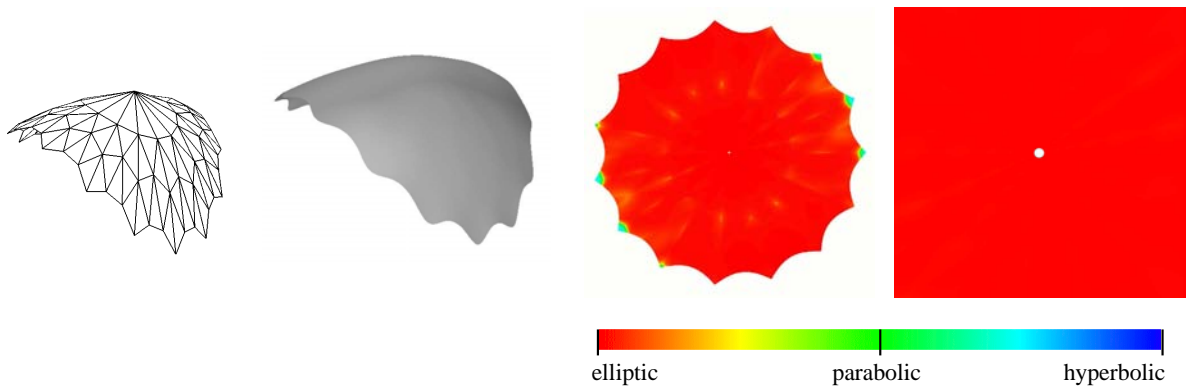
Figure 9: Control-net, flat-shaded surface and visualization of the Gauss curvature of the surface corresponding to the surface in Figure 5 corrected to an elliptic shape using \kappa_3 = 0.02 , \kappa_4 = \kappa_5 = 0 . The right column shows the zoom-in at the extraordinary point after 10 subdivision steps. Compare with the control-net and flat-shaded surface in Figure 5 and the visualization of the Gauss curvature in Figure 7 (top) of the surface with hybrid shape.
