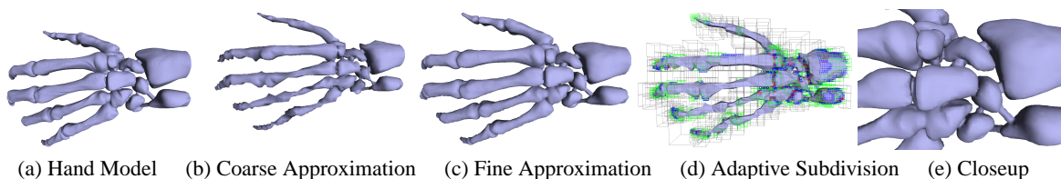
Figure 5: Topology-Preserving Simplification: Figs (a),(b),(c) show the original model along with a coarse and fine approximation generated using our topology preserving simplification algorithm. The original model has 654K triangles, while the two approximations consist of 27K and 58K triangles respectively at Hausdorff error bounds of 1 and 1/128. Fig (d) shows the adaptive grid generated for the coarse approximation. The colors, green, blue, and red in that order, indicate the increasing level of subdivision. Fig (e) shows a closeup view of a part of the fine approximation. It highlights the features in the original model and our algorithm is able to reconstruct all these features accurately. It took 36 secs to generate the approximation.
