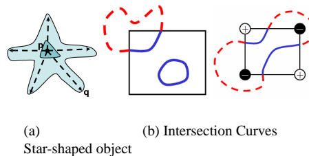
Figure 3: Fig. (a) shows a star-shaped primitive and its kernel (shaded region in the middle). P is an origin of the kernel. Fig (b) supports proof of Lemma 1. It shows a grid cell face F and the intersection of the exact surface \mathcal{E} with F . The figure on the left shows the intersection curve (in blue) consisting of two curve components, one of which is closed. As a result, it is not star-shaped. The figure on the right shows the case where the curve has two boundary curves. This results in a face ambiguity.
