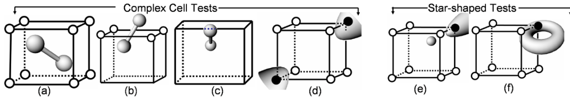
Figure 2: This figure shows the different cases corresponding to the complex cell and star-shaped test. Figs (a), (b), (c) and (d) show cases of complex voxel, complex face, complex edge, and topological ambiguity. The white and black circles denote positive and negative grid points respectively. Fig. (e) shows the case where the surface is not star-shaped w.r.t a voxel. In Fig (f), the restriction of the surface to the right face of the cell is not star-shaped.
