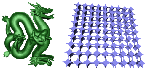
Figure 6: Boolean operations on complex models and curved primitives: The left figure shows the result of the union of two dragons. Each dragon is represented using 850K triangles. Our algorithm computes a topology preserving approximation of the final boundary. It took 95 secs to compute an approximation with 118K triangles at a Hausdorff error bound of 1/128 . The right figure shows the result of 100 difference operations between a polyhedron and 100 ellipsoids. The resulting surface has a complex topology; it has a genus of 208. Our algorithm took 16 secs to generate an approximation with the correct topology at a Hausdorff error bound of 1/64 .
