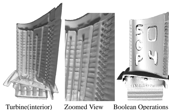
Figure 1: This 1.7M triangle model of a turbine has a high genus and many holes in the interior. We highlight the application of our novel topology preserving voxelization, simplification and boundary evaluation algorithms on this complex model. The simplified model of the turbine has 511K triangles and we show a zoomed view in the center image. We perform five difference (Boolean) operations on the turbine model and reconstruct the boundary of the final solid. Our boundary evaluation algorithm preserves the topology of the final solid and accurately computes all the components. Overall, our algorithm can perform such geometric computations on complex models in tens of seconds and give rigorous guarantees in terms of preserving the topology of the final surface.
