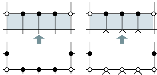
Figure 6: Phase one chain advances. Left: type one. Right: type two. Empty circles indicate corner vertices before the advance, filled circles indicate interior chain vertices.
