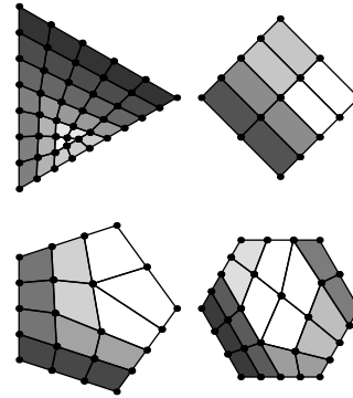
Figure 8: Various quadrangulations produced by our method. Successive phase one chain advances are shaded from dark to light.
