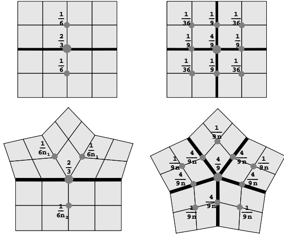
Figure 2: Change of basis mask M for an interior vertex of q^0 (top-left), a corner vertex of q^0 of valence four (top-right), a general interior vertex (bottom-left) and a corner vertex of valence n (bottom-right). Lofted edges are shown in bold.
