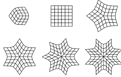
Figure 11: Characteristic map of the surface scheme for n = 3 \dots 8
