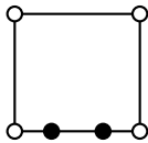
Figure 5: A patch with four corners which cannot be quadrangulated without adding extraordinary vertices. Empty circles mark the corner vertices, i.e. vertices where multiple curves meet, filled circles mark interior boundary vertices.
