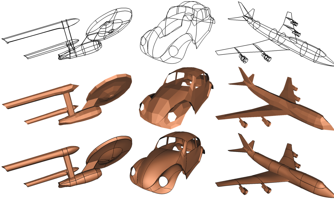
Figure 9: Examples of surfaces lofting curve networks. Each surface was computed automatically using skinning and fairing.
