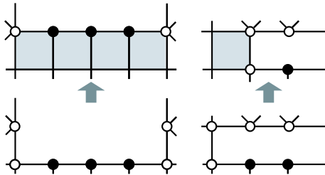
Figure 7: Phase two chain advances. Left: type three. Right: type four. Empty circles indicate corner vertices before the advance, filled circles indicate interior chain vertices.
