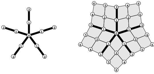
Figure 10: Block ordering for vertices on a curve network (left) and its corresponding surface mesh (right)
