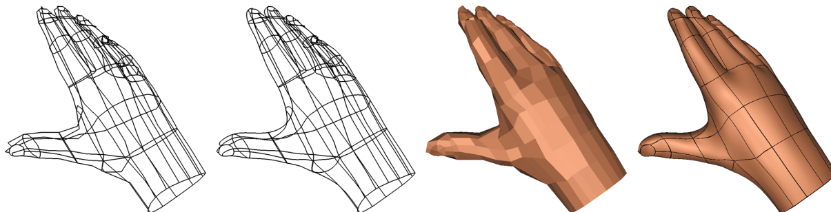
Figure 1: A network of polygonal lines q^0 and its associated curve network q^\infty (left). The base mesh p^0 for a modified Catmull-Clark surface whose limit surface p^\infty (right) interpolates q^\infty . p^0 was automatically computed from q^0 using a combination of skinning, fairing and lofting.
