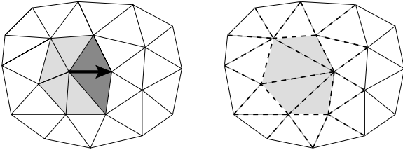
Figure 7: When an edge is collapsed (black arrow), the triangles or tetrahedra that share the edge are removed (dark gray) and the elements that touch the deleted vertex are deformed (light gray). Since the collapse weight of an edge includes data about element shape, the weight of all edges that share a vertex with a deformed element (dashed lines) must be recomputed.
