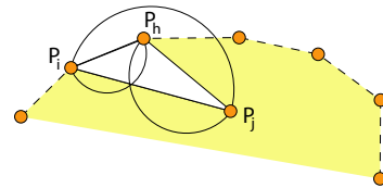
Figure 18: 2D convection property : A discovered half-edge \widehat{P_i P_j} must have its coupled half-edge meet the Gabriel property also, otherwise it could not have been inserted in the evolving surface
