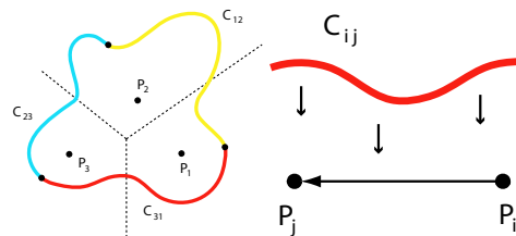
Figure 3: Decomposition of C into pieces going through d = 2 adjacent Voronoi cells only
