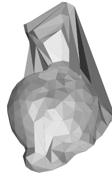
Figure 8: Sculpture result : We have added topological constraints and a priority queue to turn our algorithm into a sculpture algorithm. The weight of a half-facet can be seen as some measure of the Gabriel property. The original shape could not be extracted because the algorithm got stuck by topological constraints.
