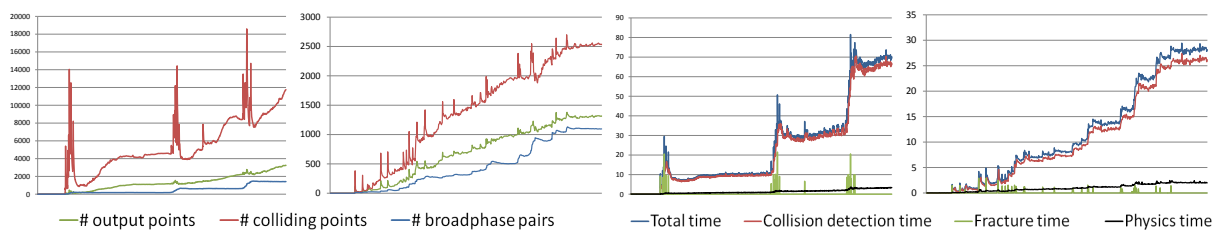
Figure 12: Plots for the ‘drop bunnies’ scene (first and third plots) and the ‘bricks’ scene (second and fourth plots). The two left plots show collision detection statistics: number of points output by adaptive collision detection (green), number of actual colliding points (red), and pairs of bodies output by broad-phase collision detection (blue). The two right plots show timings per time step: total (blue), collision detection (red), fracture computation (green), and physics computations (black). Times to update collision detection data structures were always shorter than fracture computation, and are not included for clarity.
