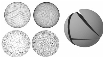
Figure 8: Sphere used for the analysis of sampling resolution on update and query costs. The top left images show two different samplings of the surface, and the bottom left images show two different samplings of the interior.
