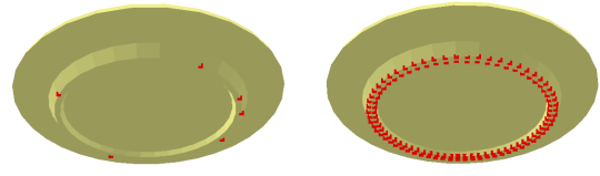
Figure 5: Rolling plate on a transparent ground, with contacts output by (left) our self-adapting collision detection (up to 6), and (right) full collision detection (up to 128). See the accompanying video.
