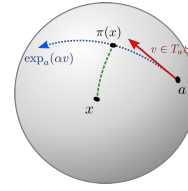
Figure 2: The geodesic projection of point x over the pose geodesic \exp_a(\alpha V) (blue) corresponds to the point where the geodesic segment in green has minimal length.
