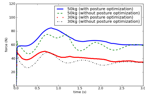
Figure 8: Forces applied by the hand on the storage cabinet.
