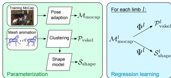
Figure 2: Analysis phase of presented method (Sec. 4).
