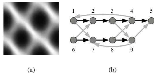
Figure 4: Motion Graph construction. (a): Transition matrix. The entry at (i,j) contains the transition value from node i to node j . Bright values indicate good transitions and dark values indicate poor transitions. (b): A simple motion graph. Black edges are from the motion clips and gray edges are created through the similarity measurement. The largest strongly connected component is \{1,2,3,4,7,8,9\} .
