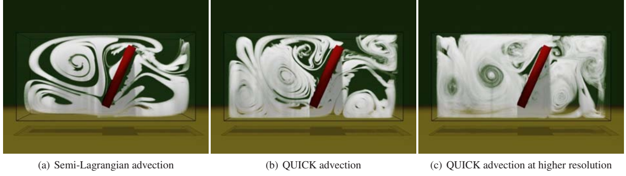
Figure 2: Smoke stirred by a paddle. Panel (a) is produced using semi-Lagrangian advection on a 64 \times 32 \times 32 grid. The large amount of numerical viscosity suppresses the naturally occurring unstable motions in the flow, leading to a smoke field that is highly filamented but without smaller scales in the flow. Panels (b) and (c) are produced using QUICK advection on grids of the same and higher resolution ( 128 \times 64 \times 64 ) respectively. Especially in panel (c), natural instabilities are no longer suppressed and the flow field exhibits a naturally turbulent field containing many scales.
