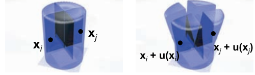
Figure 2: Crack Surfaces. A crack defines a discontinuity in the mapping from material coordinates \mathbf{x} (left) to the deformed state \mathbf{x} + \mathbf{u}(\mathbf{x}) in world coordinates (right). Shape functions in meshless discretization methods must account for these discontinuities.
