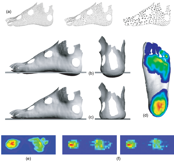
Figure 9: Contact of a deformable human foot with a rigid ground plane. (a) sampling patterns of the hierarchical representation used for collision detection and multi-level computations, (b) original, undeformed configuration, (c) final deformed surface, (d) normal tractions on foot, (e) normal tractions on ground plane, (f) measured tractions. Blue denotes zero traction and red maximum traction.
