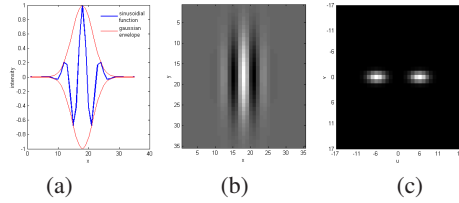
Figure 1: Gabor Filter with \sigma = 3.37 , \theta = 0 , \lambda = 6 , \gamma = 0.5 and \phi = 0 . (a) Scan along the x -axis showing the sinusoidal function superimposed upon the Gaussian envelope, (b) the Gabor filter in the space domain, (c) the power spectrum of the filter.
