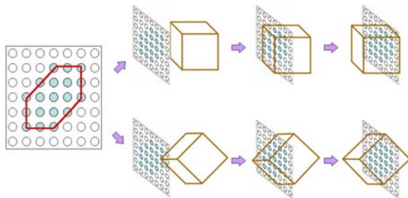
Figure 4: Computational mask.
