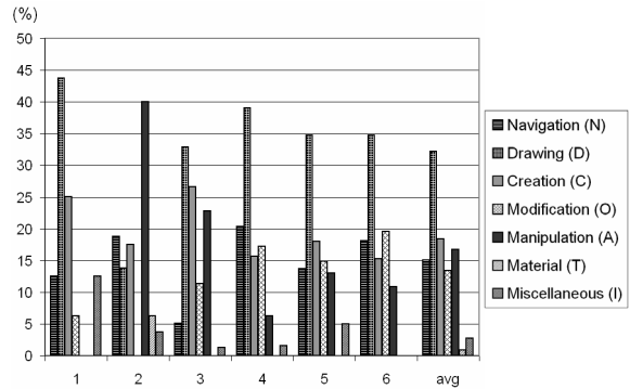
Figure 5: Percentage of operation categories by user
