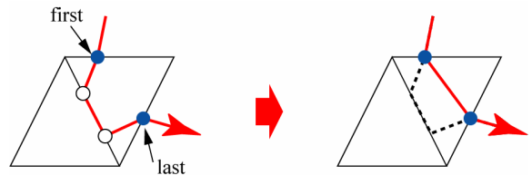
Figure 8: A stroke crosses a triangle multiple times.
