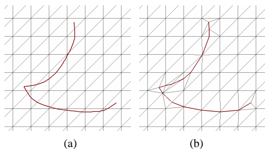
Figure 16: Result for a stroke that contains a sharp angle.
