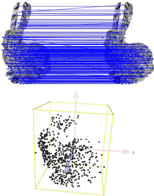
Figure 3: 3D Estimation on a Stanford Bunny with stereo images: Top image illustrates the SURF Stereo matching were features are detected and their descriptor is used to find the correspondences between features in the images. Bottom image is the resulting sparse 3D point cloud.
