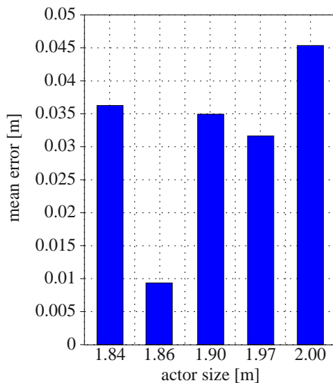
Figure 5: Results of test with actors of different sizes. We plot the mean reconstruction error for a walking sequence (HDM_**_01_01_01_120.C3D) versus the body size of the actors. The actors were not included in the database for this experiment.
