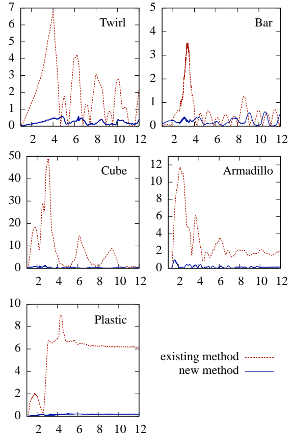
Figure 2: The measured volume error in % (y-axis) over time in seconds (x-axis) for both methods in all examples.
