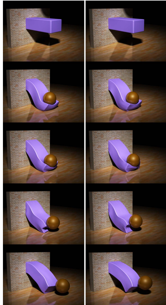
Figure 4: Using a strong distance stiffness can prevent too much volume loss in the existing method (left). Still the new method (right) can better reduce the volume loss.
