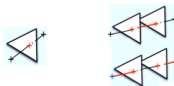
Figure 4: Left: Intersected vertices step , an intersection vertex (in red) between an edge and a facet. Right: Restricted edges step , two situations where restricted edges (in red) are created using original edges (in blue) and intersected vertices (in red).
