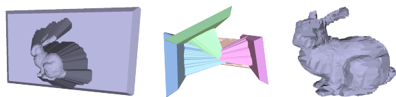
Figure 6: Bunny with 4 depth cones. In order: one input depth cone, all input depth cones intersecting, visual cropping intersection output.
