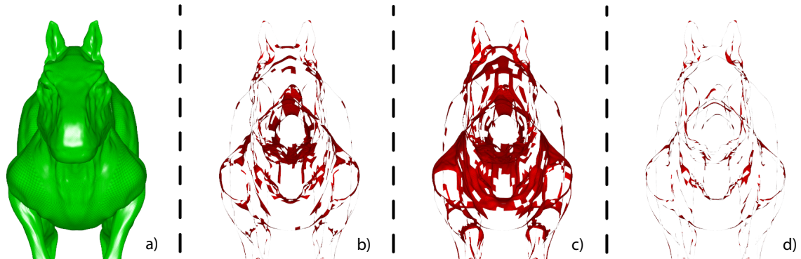
Figure 1: The killeroo (a, 11532 Bézier patches), is rendered with different strategies for back-patch culling. For each algorithm we visualize wasted computations: areas processed by the tessellator but back-facing and hence not visible; less area is better. The cone-of-normals (b, 3697 patches culled) is effective, but costly for dynamic scenes. Its approximation from tangent and bitangent cones is faster to compute, but less precise (c, only 2621 patches culled). Our approach is faster than the cone-of-normals, and more effective (d, 4604 patches culled).
