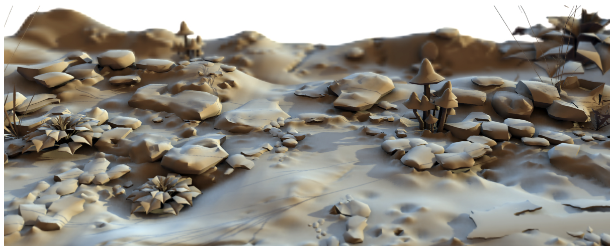
Figure 1: Possible game scenario with lighting using bent normals: 2048 \times 1024 pixels, 60.0fps, including direct light and DOF on an Nvidia GF 560Ti. Environment mapping produces natural illumination, while bent normals cause colored shadows.
