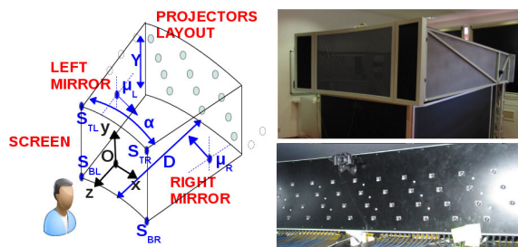
Figure 4: Test case: calibration of a cylindrical HPO display. Left: schematic layout. Right: pictures taken from the light field display HV640RC highlighting the screen layout, the projectors layout and the position of camera.
