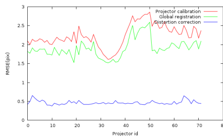
Figure 5: Comparison of accuracy after the different steps of calibration of HV640RC display. Errors (RMSE) on chessboard control points.
