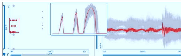
Figure 5: The results from the second iteration (the scatterplot is zoomed in). The curves are of the desired shape. Moving the subspace further to the left (smaller L_{line} ) is not possible due to the physical constraints of the system.
