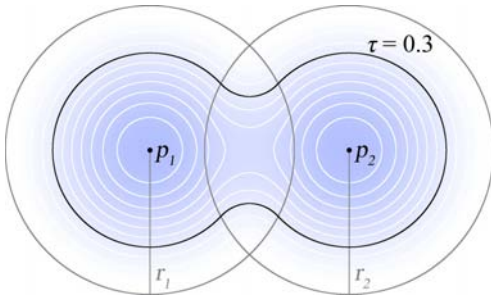
Figure 2: An implicit surface defined in \mathbb{R}^2 by two generator points p_1 and p_2 with radii of influence r_1 and r_2 and a threshold of \tau = 0.3 .
