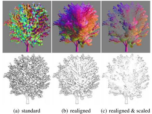
Figure 7: Application to non-photorealistic rendering. Top row: Normal buffer; normal vectors are mapped to RGB color space. Bottom row: Edge detection filter applied to the normal map.
