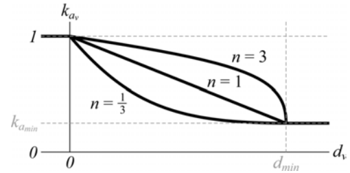
Figure 4: Dependency of the ambient reflection coefficient k_{a_v} on the density value d_v according to Equation 4 for the three different exponents n = \frac{1}{3} , n = 1 , and n = 3 .
