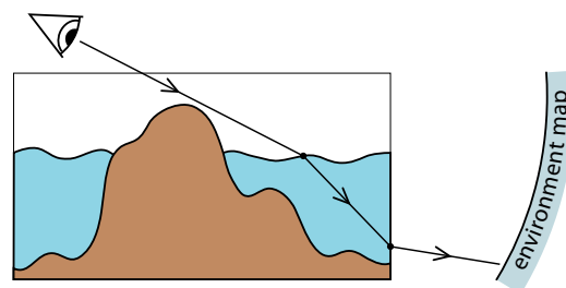
Figure 5: Outgoing light rays from an unclosed water volume. We look up an envmap to find out what they “see”.
