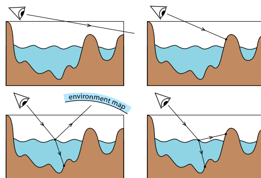
Figure 4: The algorithm handles four possible situations.
