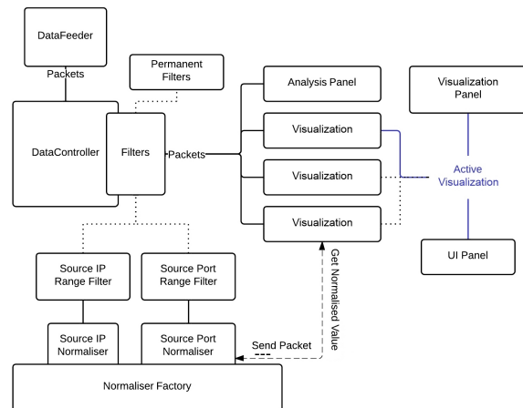
Figure 2: Diagram overviewing the architecture of NetVis.
