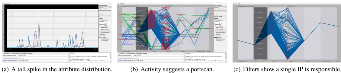
Figure 11: Example scenario of a network portscan.
