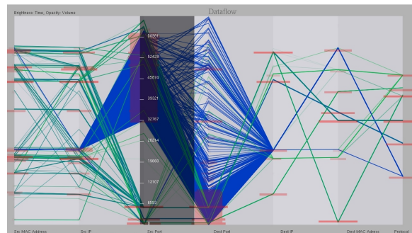
Figure 5: Data Flow visualization inspired by parallel coordinate plots [Ins85].
