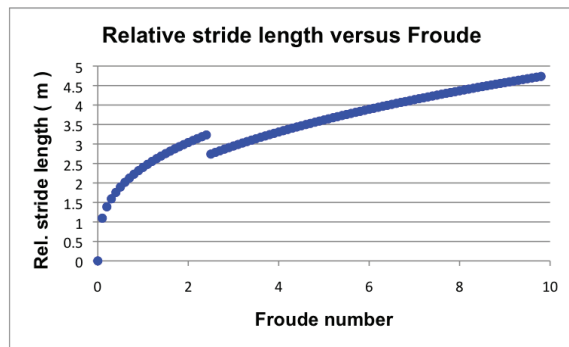
Figure 4: Relative stride length versus Froude number.
