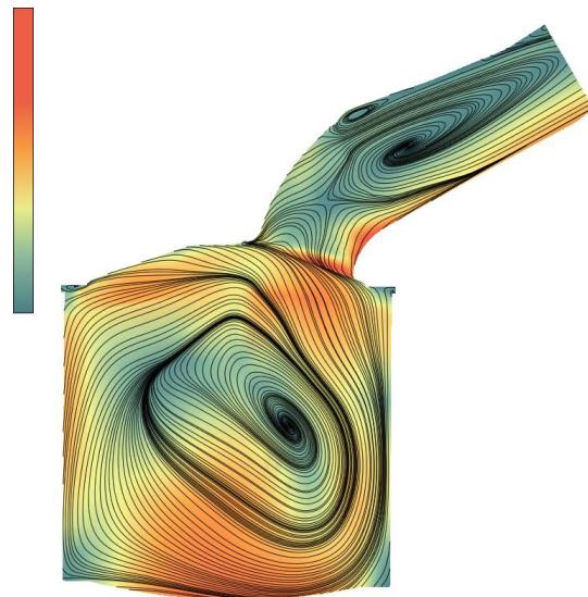
Figure 3: Visualization of flow through the gas engine simulation. By setting d_{rest} to 0.05 \times d_{sep} , streamlines overlay highlighting loops within the flow field. [SLCZ09]
