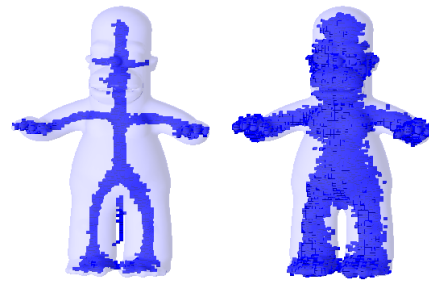
Figure 8: CGView allows to visualize discretized scalar fields in voxel grids. In the image we show two different threshold for a voxel grid computed using the algorithm in Section 3.1.
