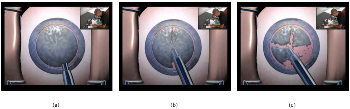
Figure 5: A virtual phacoemulsification sequence. Here we show a typical lens rupture and extraction performed by a phacoemulsification tool. The typical cross-shaped cut is clearly visible.
