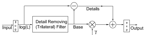
Figure 3: Contrast reduction method based on edge-preserving filters.
