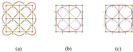
Figure 3: Threads calculated with a) Cubic hermite curves, b) B-spline curves, c) Interpolating B-splines.
