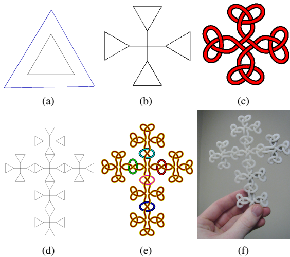
Figure 10: The encapsulation process. a) A triangle capsule with bounding volume. b) A larger capsule constructed by connecting 4 triangle capsules. c) The knot resulting from the graph of the capsule in b). d) 6 capsules from b) joined in a high cross pattern. e) The knot resulting from the graph in d). f) The high cross from e) has been fabricated.
