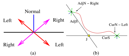
Figure 2: a) Stroke geometry. b) Thread construction example.
