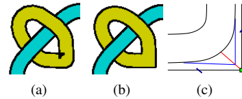
Figure 4: The interior overlap in a) has been culled in b) and the outer edge has been sharpened. c) This figure shows how we sharpen corners. The thread path is altered to follow the blue lines towards a position at some user defined distance along the vector that lies between the junction and the median of the outside curve.
