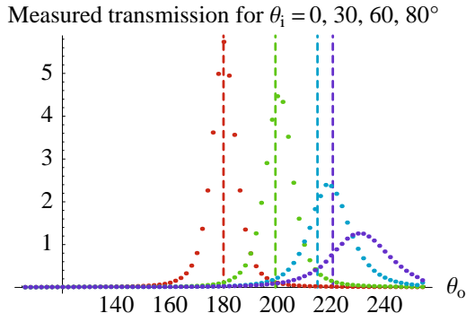
Figure 2: Measured transmission ( f_t(\mathbf{i}, \mathbf{o}, \mathbf{n}) |\mathbf{o} \cdot \mathbf{n}| ) for a rough surface (ground glass) at 0, 30, 60, and 80 degrees incidence angle. Dashed lines are the refracted directions predicted by Snell's law for a smooth surface. Note that the transmitted lobe grows broader as the incidence angle increases and is shifted significantly towards grazing compared to refraction through a smooth surface.
