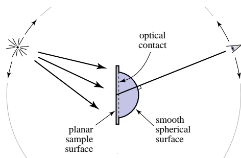
Figure 9: Measurement setup: We bonded a glass hemisphere to the back of our samples, to allow us to observe transmission even at grazing angles.
