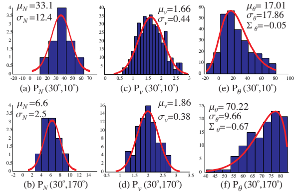
Figure 9: The splash distributions, P_N(\alpha, \phi) , P_v(\alpha, \phi) , and P_\theta(\alpha, \phi) , for the wood sample at an inclination of 30^\circ . The top row shows the splash distributions for \phi = 10^\circ (almost along the direction of inclination), while the bottom row shows the distributions for \phi = 170^\circ (almost opposite to the direction of inclination). Notice the significant variations in the splash distributions with respect to \phi . Based on previous studies, we use the Gaussian model for P_N(\alpha, \phi) and P_v(\alpha, \phi) and the generalized extreme value model for P_\theta(\alpha, \phi) .
