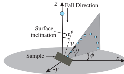
Figure 2: Parameters used to describe a splash event. The magnitude of the velocity of a droplet is denoted by v and its orientation is denoted by the elevation angle \theta and the azimuthal angle \phi . \alpha is the inclination of the surface with respect to the fall direction of the drop (gravity).
