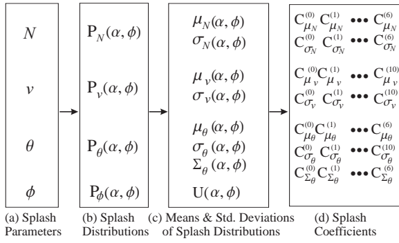
Figure 8: The pipeline used to estimate a compact splash model for each material. (a) The splash parameters (number, velocity, and orientation) measured using the structured light method. (b) A distribution is computed for each parameter, for each of the discrete values of (\alpha, \phi) . (c) We fit a probability model to each of these distributions to obtain its mean \mu and standard deviation \sigma . (d) The means and standard deviations vary smoothly with \alpha and \phi . Low-order polynomial surfaces are used to compactly represent these variations. The final splash model of a material has a total of 54 coefficients.
