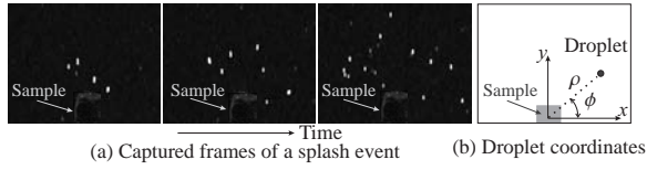
Figure 4: (a) Three frames (time instances) of a measured splash. The bright spots correspond to intersections of droplets with the light sheet. (b) \rho is the radial distance (in pixels) of the droplet from the center of impact and \phi is its azimuthal angle measured from the x -axis.
