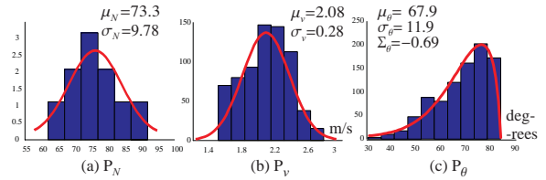
Figure 7: The splash number distribution P_N , velocity distribution P_V , and elevation angle distribution P_\theta , for the wood sample for head-on impact. We use the Gaussian model for P_N and P_V and the generalized extreme value model for P_\theta .
