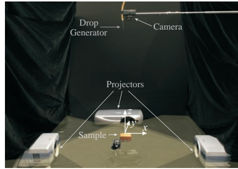
Figure 3: Apparatus used for measuring splash parameters. Three projectors are used to create a thin sheet of light below the sample material. Drops are produced using a drop generator and the sample is observed using a high-speed camera placed close to the generator. The splash droplets produce bright spots in the camera image when they pass through the sheet of light. The location and time at which each droplet passes the light sheet determines its velocity and orientation.
