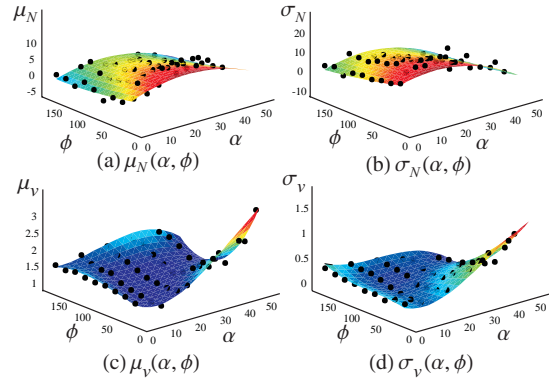
Figure 10: The black dots are the estimated means and standard deviations for (a,b) the number distributions and for (c,d) the velocity distributions for wood. While 2nd order polynomial surfaces fit the means \mu_N(\alpha, \phi) and standard deviations \sigma_N(\alpha, \phi) of the number distributions well, 3rd order polynomial surfaces are needed for the means \mu_v(\alpha, \phi) and standard deviations \sigma_v(\alpha, \phi) of the velocity distributions.
