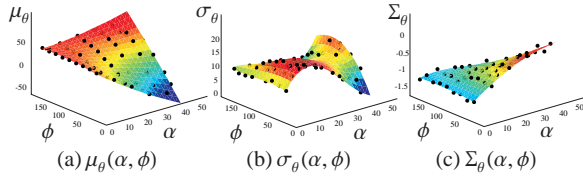
Figure 11: The black dots are the measured (a) means \mu_\theta(\alpha, \phi) (b) standard deviations \sigma_\theta(\alpha, \phi) and (c) shape factors \Sigma_\theta(\alpha, \phi) of the elevation angle distributions for the wood sample. Fits of polynomial surfaces of order 2 were used for the means \mu_\theta(\alpha, \phi) and shape factors \Sigma_\theta(\alpha, \phi) , while a surface of order 3 was used for the standard deviations \sigma_\theta(\alpha, \phi) .
